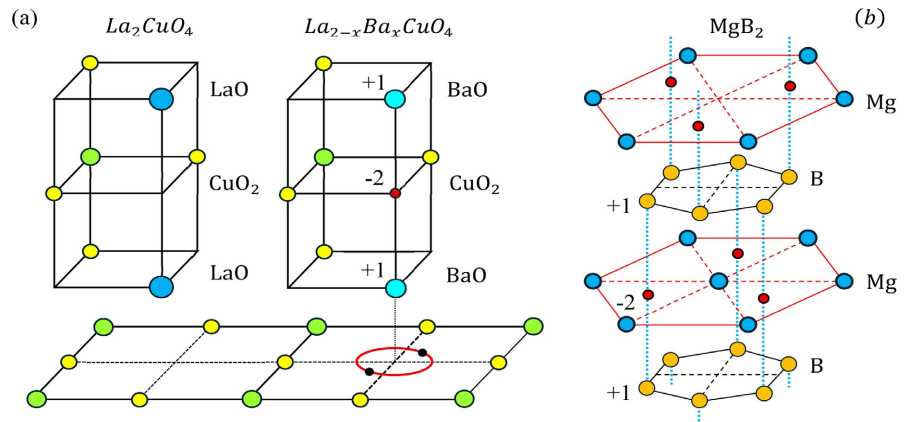
Figure 12. (a) Unit cell of layered copper oxides, where one or two La atoms can be replaced by a Ba atom, but an electron-pair is then formed in the void of the intermediate \text{CO}_2 plane. (b) \text{MgB}_2 crystals are also medium HT superconductors because of Coulomb forces.
