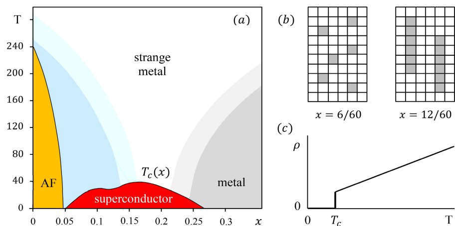
Figure 13. (a) Phase space for \text{La}_{2-x}\text{Sr}_x\text{CuO}_4 for different values of the absolute temperature T and doping x . The superconductive state is limited to the red domain. (b) There are two possible distributions of doped cells. (c) At about optimal doping, the electrical resistivity \rho increases in a linear way for increasing temperatures T > T_c .
